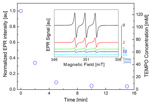
Fig. 4 EPR monitoring of the TEMPO concentration for the reaction of C18 with 4 mol% TEMPO and 2 mol% DCP at 150\text{ }^\circ\text{C} : TEMPO-normalized EPR intensities ( I/I_0 = I(t)/I(t=0) ) were obtained at t = 0, 2, 5, 10 and 15 min with corresponding EPR signals (inset).
