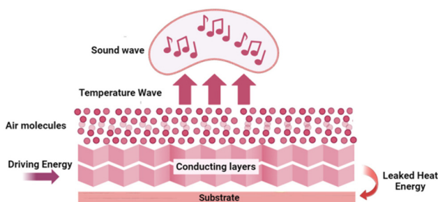
Fig. 10 Working principle of a thermoacoustic sound source, created with BioRender.com.
