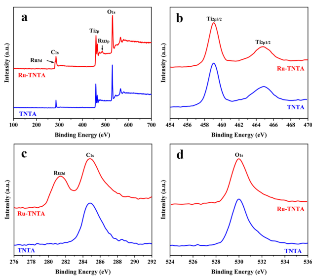
Fig. 2 XPS spectra of TNTA and Ru-TNTA (a: full spectrum, b: Ti_{2p} , c: Ru_{3d} , and d: O_{1s} ).
