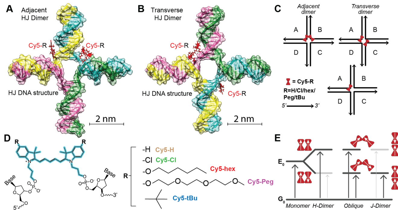
Fig. 1 (A) Schematic of AB adjacent homodimer. Dye position (A) represents initial localization based on base pair site and not the position adapted upon dimer formation. (B) Schematic of AC transverse homodimer. Dye position (B) represents initial localization based on base pair site and not the position adapted upon dimer formation. (C) Simple line schematic of the representative HJ structures. Black lines in this case represent the DNA, with the arrow denoting the 5' to 3' direction, and red bowtie the Cy5-R dye. We note that adjacent dimers can be represented: [AB, BC, CD, or AD] while transverse dimers: [AC and BD]. Monomers include the [A, B, C, and D] conformations. (D) Chemical structure of the Cy5-R showing the two-point attachment to DNA. The R groups are shown to the right. (E) Schematic of the TDM alignments and coupling of the energy levels in the dimers. Red bowties as in C, while the white arrows represent the TDM alignment. The upward arrows indicate absorptive transitions from the ground state, where a dark grey arrow indicates an allowed transition and a light grey arrow indicates a forbidden transition.
