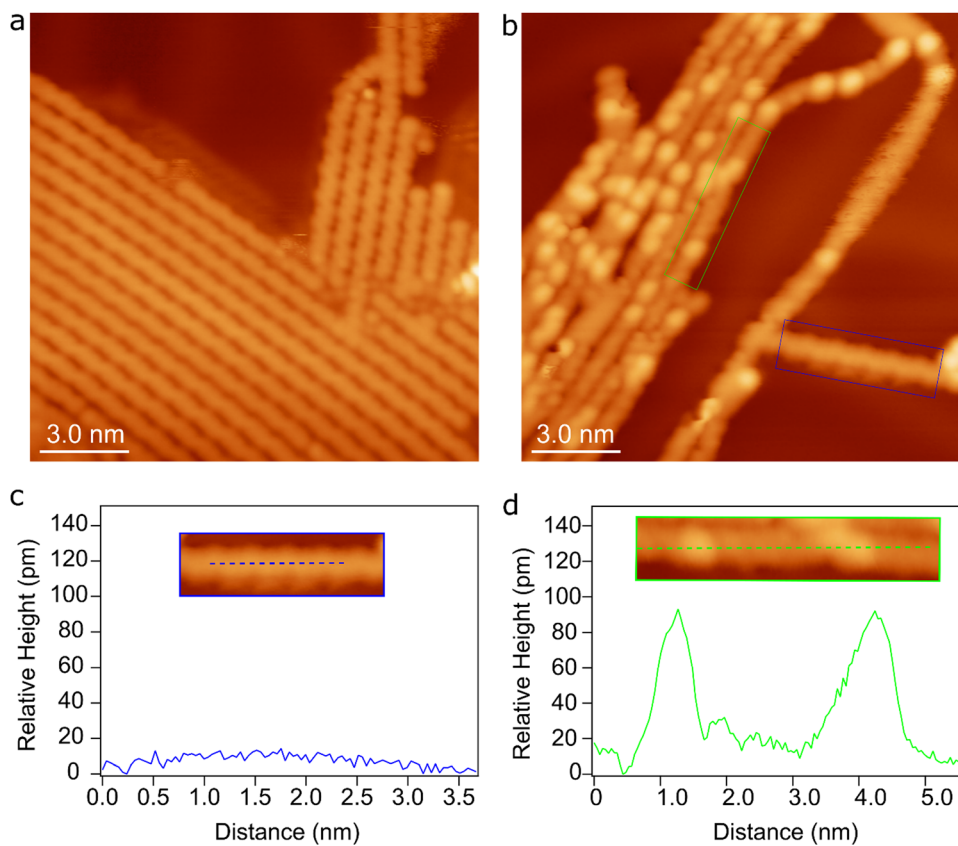
Fig. 8 STM images taken after deposition of a submonolayer of 4,4''-dibromo-2,2',2'',5,5',5''-hexafluoro-1,1':4',1''-terphenyl onto Au(111) followed by annealing to (a) 473 K and (b) 600 K. Tunneling parameters: (a) U = -1.8 V, I = 0.17 nA; (b) U = -0.5 V, I = 0.25 nA. (c) and (d) show the apparent height profiles along the blue and green line in the insets, which are cut out from panel (b) as marked by the blue and green rectangles.
