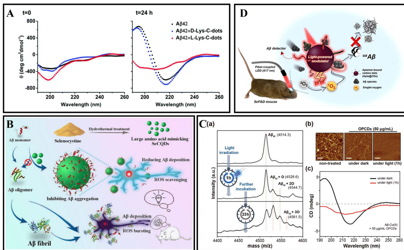
Fig. 13 (A) Secondary structures of 25 mM A \beta_{42} monitored by CD spectroscopy in the absence or presence of D-Lys-C-dots or L-Lys-C-dots. 219 (B) Synthesis of SeCQDs and the inhibition effects of SeCQDs on A \beta aggregation and ROS production. 221 (C): (a) The mass spectra of A \beta -Cu(II) aggregates incubated with OPCDs for 24 hours at 37 °C. Light was irradiated only for one hour. (b) AFM images and (c) CD spectra of A \beta -Cu(II) aggregates incubated with OPCDs under dark and one-hour-light illuminating conditions. 232 (D) A \beta -targeting, CD-mediated photodynamic modulation for spatiotemporal inhibition of A \beta aggregation in vivo . 229
