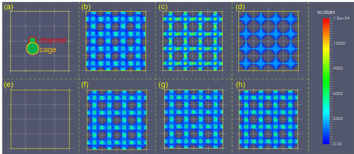
Fig. 9 The ethanol adsorption density distribution of W_s in l = 7.5 \text{ \AA} 4 \times 4 \times 4 supercell with fixed \varepsilon = 2.52 \text{ kJ mol}^{-1} for (a) \sigma = 1 , (b) \sigma = 2 , (c) \sigma = 3 , and (d) \sigma = 4 \text{ \AA} . The ethanol adsorption density distribution of W_s in l = 7.5 \text{ \AA} 4 \times 4 \times 4 supercell with fixed \sigma = 2.2 \text{ \AA} for (e) \varepsilon = 0.42 , (f) \varepsilon = 1.68 , (g) \varepsilon = 2.94 , and (h) \varepsilon = 4.2 \text{ kJ mol}^{-1} .
