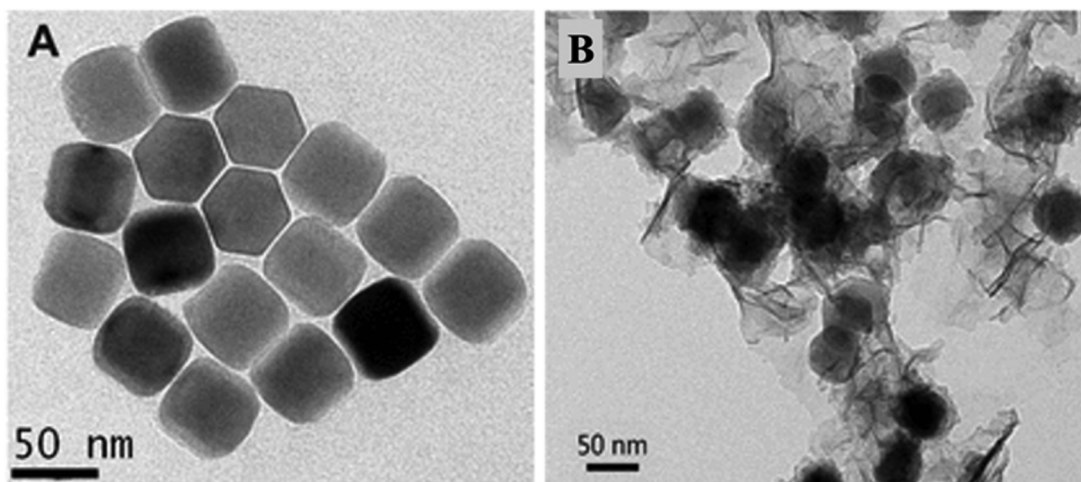
Fig. 13 TEM images (A) of OA-capped NaYF 4 :Yb,Tm@NaYF 4 core shell UCNPs, and (B) of MnO 2 NS-modified NaYF 4 :Yb,Tm@NaYF 4 UCNP assemblies. 67 Copyright©2015, American Chemical Society.
