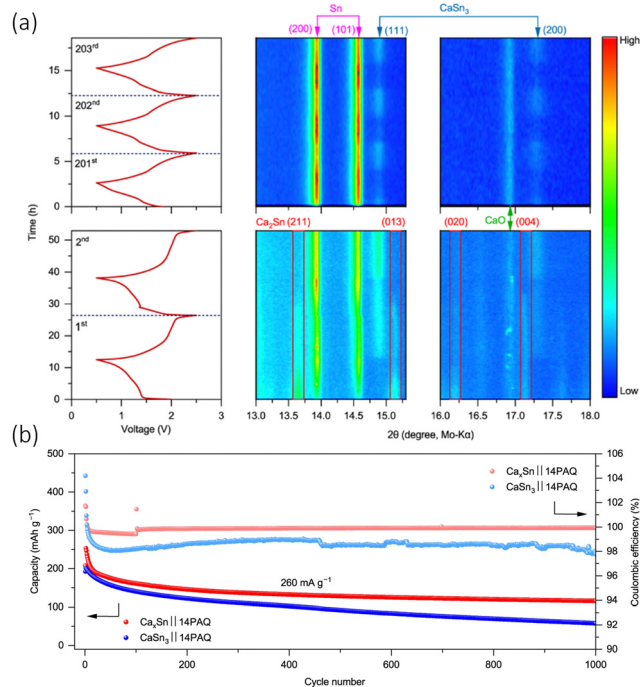
Fig. 8 (a) Isoplots of in situ XRD scans the anode Ca x Sn||14PAQ cells during the first, second and from 201 st to 203 rd discharge/charge cycles at specific current of 26 mA g -1 at 25 °C. The peak is observed along the top and the cell voltage profiles on the left had side. ICSD-ID: Ca 2 Sn 659 611, β-Sn 106 072, CaSn 3 58 934, Ca 36 Sn 23 54 619 and CaO 26 959. (b) Cycling performance of CaSn 3 ||14PAQ compared with Ca x Sn||14PAQ. Reproduced with permission from ref. 94, copyright 2022 Springer Nature.
