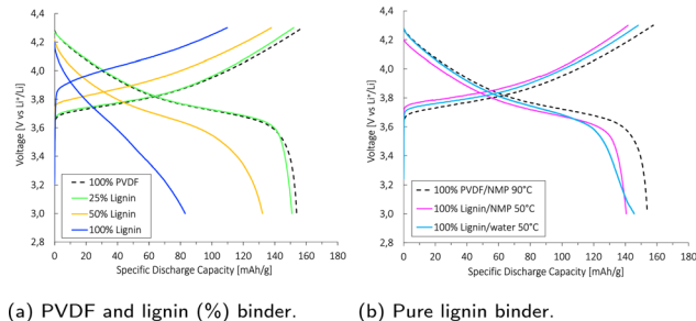
Fig. 8 Specific discharge capacity during the third formation cycle at C/10 (1C = 160 mA g -1 ). The cathodes were coated onto Al-foil with a mass loading of 4.4–4.8 mg cm -2 , and calendered at P_{\text{medium}} . A PVDF/NMP-based cathode dried at 90 °C (black) was used as a baseline. The cathodes were cycled between 3.0 and 4.3 V (vs. Li + /Li) against a Li-metal anode in a coin cell at 22 °C.
