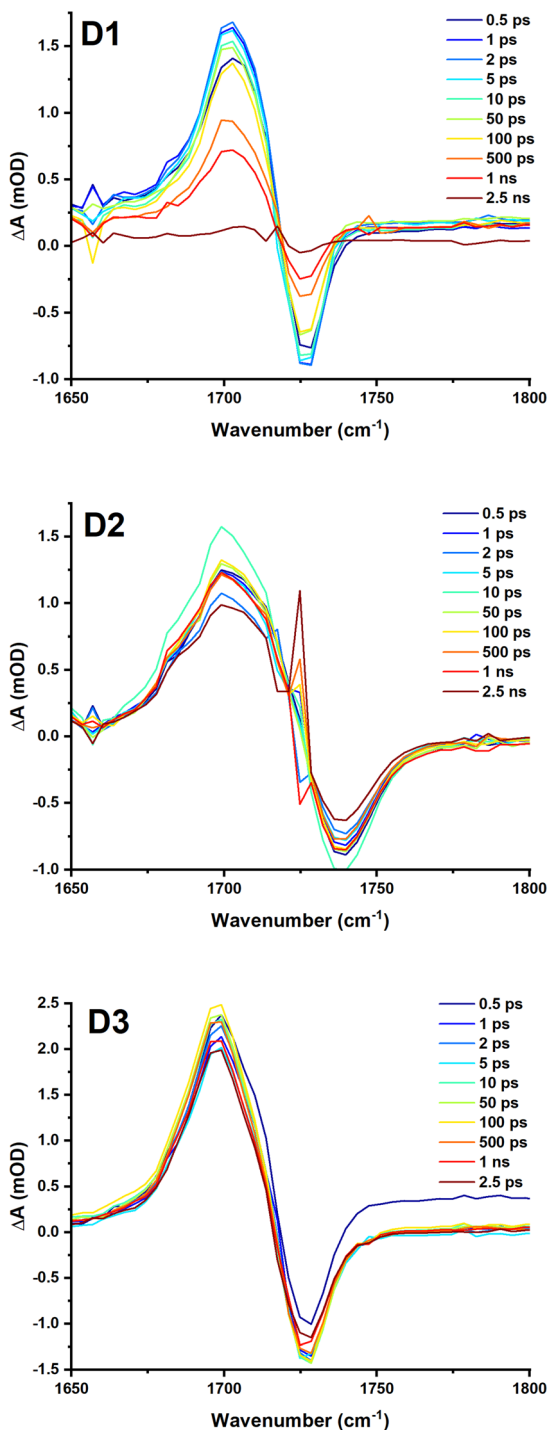
Fig. 8 TRIR spectra of D1, D2 and D3 in DCM following excitation at 525, 500 and 500 nm respectively (2 mW, \text{OD@}\lambda_{\text{ex}} \approx 0.6 ), collected with the pump set to magic angle ( 54.7^\circ ) with respect to the probe. The time delay between the pump and probe for each spectrum is shown in the legend. Kinetic traces are shown in the ESI.†
