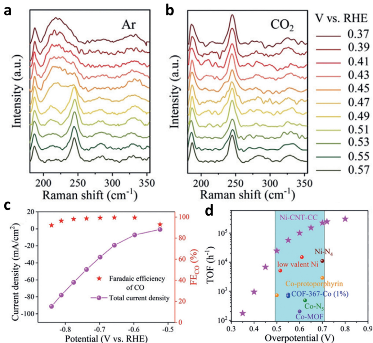
Fig. 16 (a and b) Raman spectra of Ni-TAPc collected on an Au electrode at various potentials under (a) Ar (1.0 atm) and (b) CO 2 (1.0 atm). Electrochemical performance: (c) FE CO and J_k at different potentials acquired on a carbon cloth electrode in CO 2 -saturated 0.5 M KHCO 3 solution. (d) The TOF of Ni-CNT-CC (Ni-CNT represents Ni-TAPc anchored on carbon nanotubes) compared with those of other CO 2 -to-CO reduction catalysts. Reproduced with permission. 113 Copyright (2020) Wiley-VCH.
