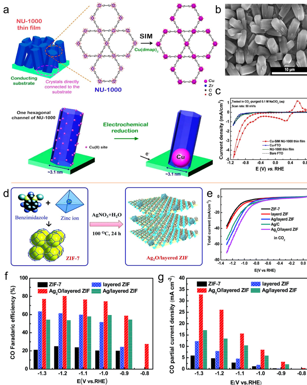
Fig. 15 (a) Schematic representation of installation of SIM in \text{Cu}(\text{II}) single site. (b) SEM image of NU-1000 film. (c) CV curves. Reproduced with permission from ref. 172 Copyright 2017, ACS. (d) Schematic synthesis of \text{Ag}_2\text{O}/\text{layered ZIF} . (e) LSV curves and (f) FEs for CO. (g) CO partial current densities vs. E . Reproduced with permission of ref. 173 Copyright 2017, RSC.
