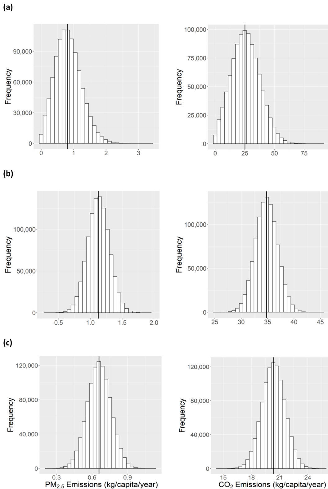
Fig. 2 Particulate matter ( PM_{2.5} , left) and carbon dioxide ( CO_2 , right) annual emission estimate distribution from Monte Carlo samplings for (a) the Xalapán region of Jalapa, (b) the city of Jutiapa, and (c) Guatemala city.
