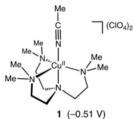
Fig. 1 Structure of complex 1 . Reduction potential of 1 (vs. Fc/Fc + in acetonitrile) is shown in parentheses. The cyclic voltammogram of 1 is presented in Fig. S2.†
