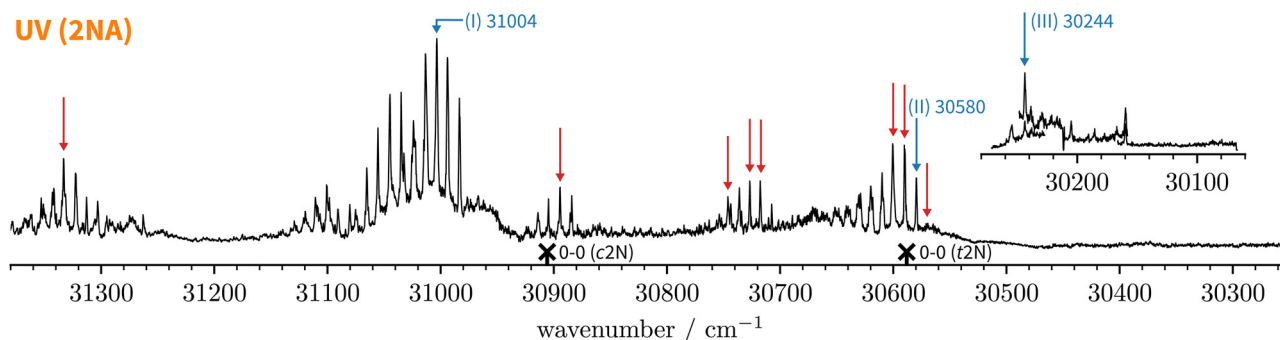
Fig. 5 Normalised one-colour REMPI spectrum of the jet-cooled co-expansion of 2-naphthol and anisole monitored at the 2NA mass channel (252 amu). The 0-0 band positions of the S_1 \leftarrow S_0 transitions of c2\text{N} and t2\text{N} are shown for reference (crosses). The normalised LIF spectrum below 30\,280\text{ cm}^{-1} is shown as an inset. Blue arrows mark selected S_1 \leftarrow S_0 transitions where IR-UV double-resonance spectra were recorded (see Fig. 6). Red arrows mark all S_1 \leftarrow S_0 bands that were checked to exhibit the same IR spectrum as bands (I) and (II).
