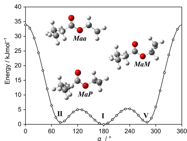
Fig. 5 The potential energy curve of ethyl butyrate obtained by a rotation about the O3–C14 bond in a grid of 10°. Calculations were performed at the MP2/6-311++G(d,p) level. The energies are given relative to the lowest energy conformation. Maa: conformer I; MaP: conformer II, MaM: conformer V.
