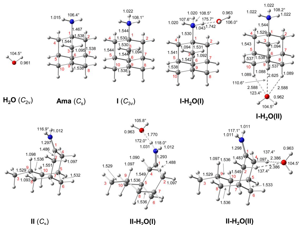
Fig. 1 Calculated equilibrium structures (in Å and degrees) of \text{H}_2\text{O} , Ama, \text{AmaH}^+(\text{I,II}) , and \text{AmaH}^+(\text{I,II})(\text{H}_2\text{O})(\text{I,II}) in their ground electronic state (B3LYP-D3/cc-pVTZ). All bond lengths are shown in ESI† (Fig. S22).
