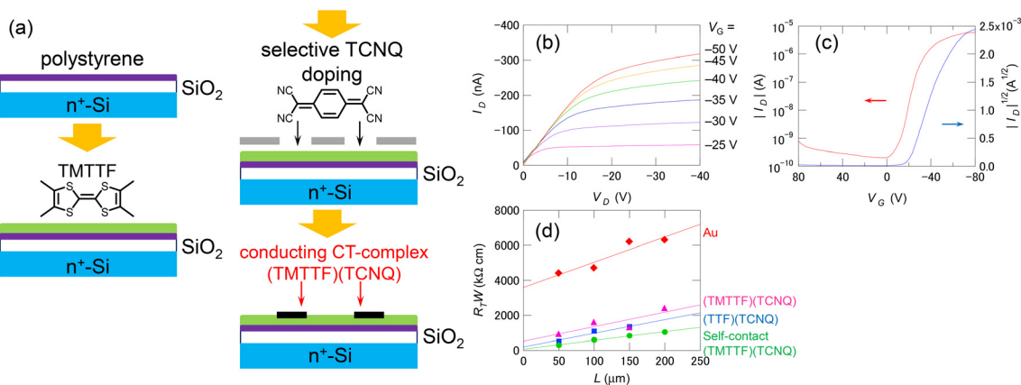
Fig. 4 (a) Schematics of the fabrication procedure of the chemical-doped self-contact transistors. (b) Output and (c) transfer characteristics of a self-contact transistor based on TMTTF/(TMTTF)(TCNQ). (d) Channel length dependence of the total resistance R_T normalized with respect to the channel width W for the top-contact transistors. Reprinted with permission from ref. 97. Copyright 2013, AIP Publishing.
