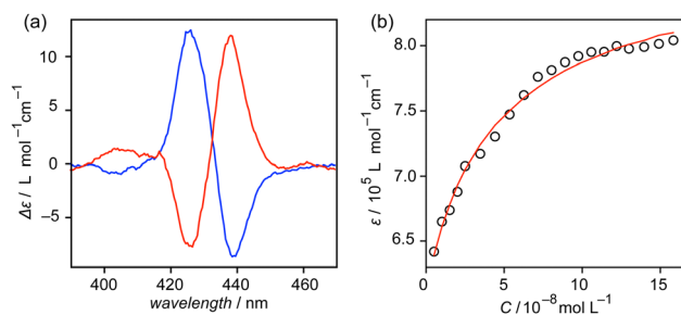
Fig. 3 (a) ECD spectra of 2 (2.5 × 10 -5 mol L -1 ) in (red) (+)-limonene and (blue) (–)-limonene at room temperature. (b) Binding isotherm analysis corresponding to the formation of intermolecular bis(porphyrin)–bis(porphyrin) self-complementary pairs of 2 in an iterative fashion in (+)-limonene at 90 °C. The plotted extinction coefficient ( ε ) values are λ = 435 nm. The full spectra are shown in Fig. S7 (ESI † ).
