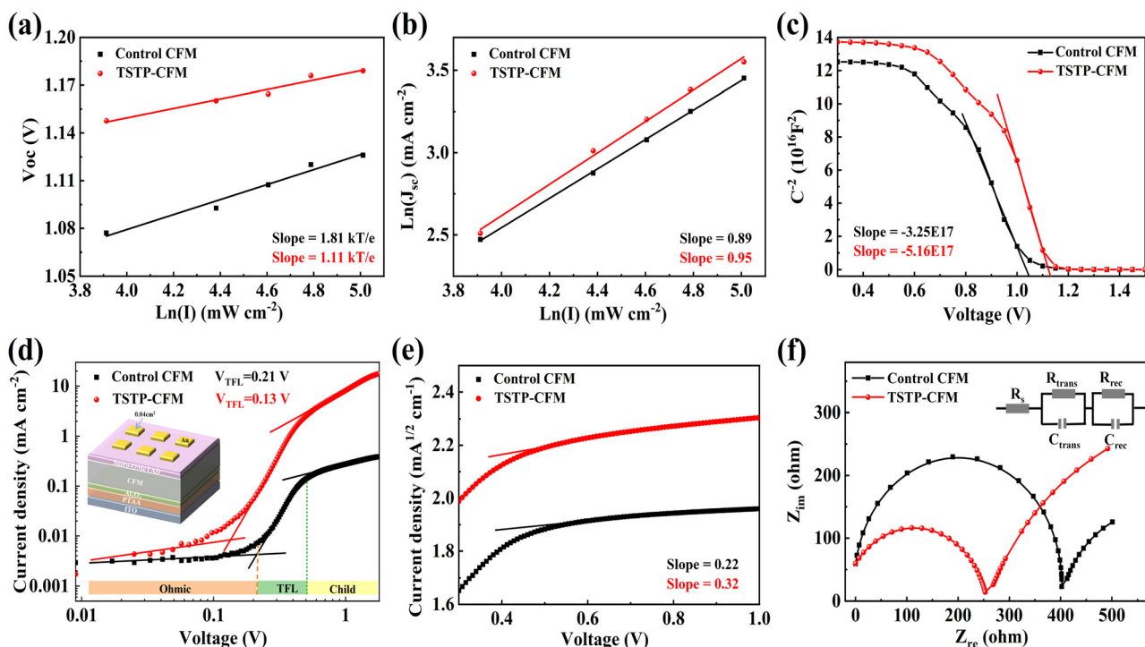
Fig. 6 (a) V_{oc} and (b) J_{sc} versus light intensity and (c) M-S plots of the control CFM and TSTP-CFM devices. (d) J-V and (e) J^{1/2}-V characteristics of SCLC measurements for hole-only devices with the architecture of ITO/PTAA/CFM (with and without TSTP treatment)/spiro-OMeTAD/Au; the inset is the device structure diagram. (f) EIS of the control CFM and TSTP-CFM devices under the illumination of 100\text{ mW cm}^{-2} ; the inset shows the equivalent electrical circuit of PSCs.
