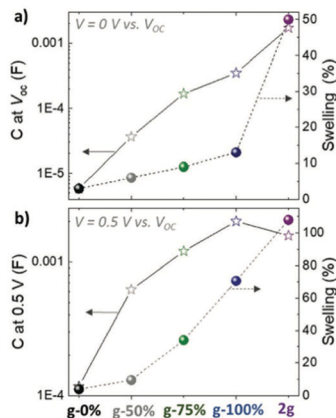
Fig. 11 The swelling behaviour and volumetric capacitance with respect to different glycol fractions in p(g2T-TT) and 2g based polymers at (a) V = 0 V and (b) V = 0.5 V versus V_{OC} . Reproduced from ref. 79 with permission from Wiley-VCH.
