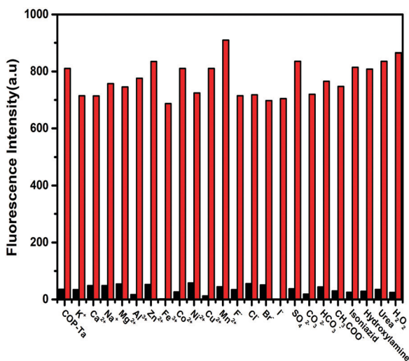
Fig. 5 Comparison of the fluorescence intensity of COP-Ta in the presence of various interfering components (100 \mu M) in water before (black bar) and after (red bar) the addition of hydrazine (200 mM).
