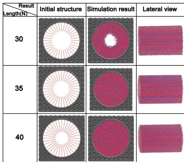
Fig. 7 Morphologies of nanopores with different chain lengths at high salt concentrations.
