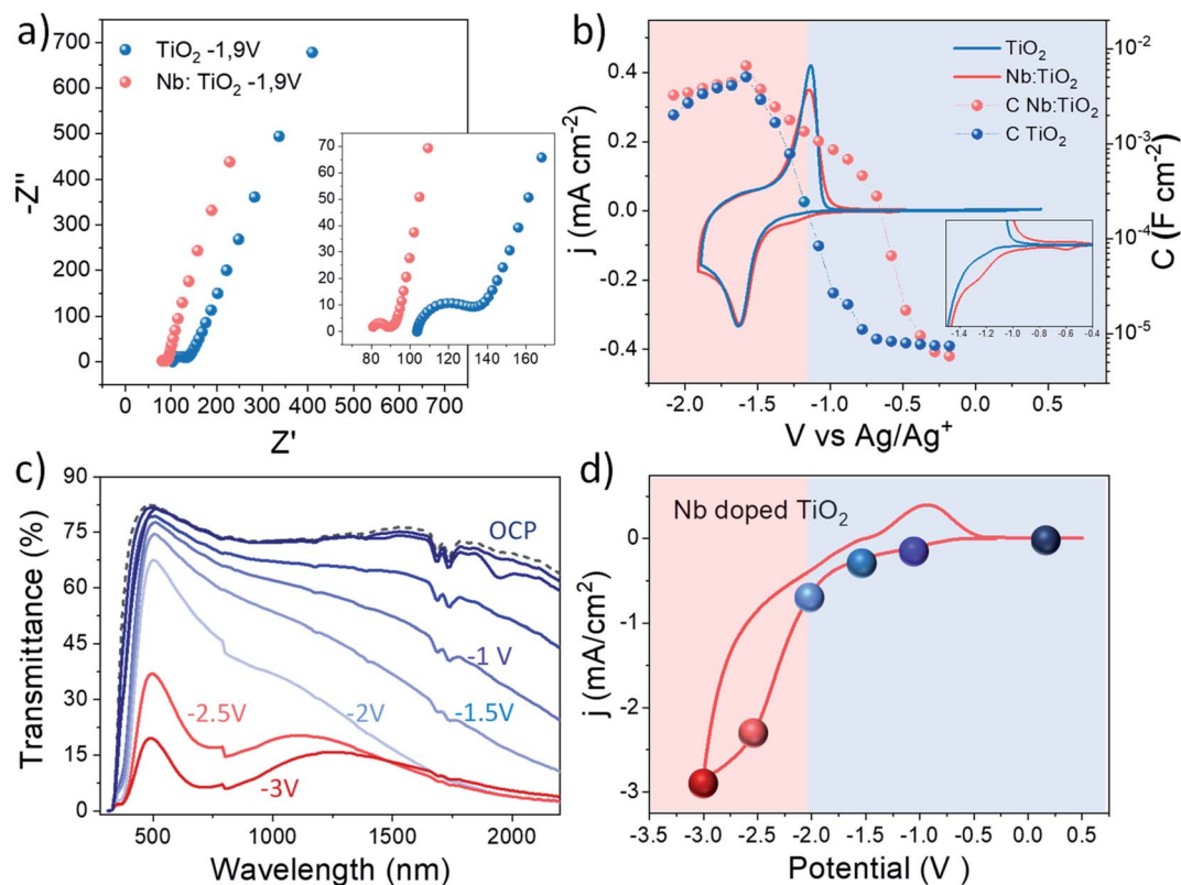
Fig. 5 (a) Nyquist Plot of bare and Nb doped \text{TiO}_2 at -1.9\text{ V} vs. \text{Ag}/\text{Ag}^+ . (b) Cyclic voltammetry (solid lines) and charge capacitance (balls) associated with the different potential points of \text{TiO}_2 (blue) and Nb-doped \text{TiO}_2 (red). (c) Transmittance spectra and (d) cyclic voltammogram of a lab-scale device of Nb doped \text{TiO}_2 at 50\text{ mV s}^{-1} . The spheres represent the potential points at which the transmittance measurements of the device have been carried out.
