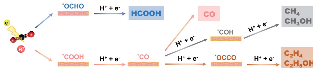
Fig. 2 Different pathways for the electrochemical \text{CO}_2\text{RR} .
