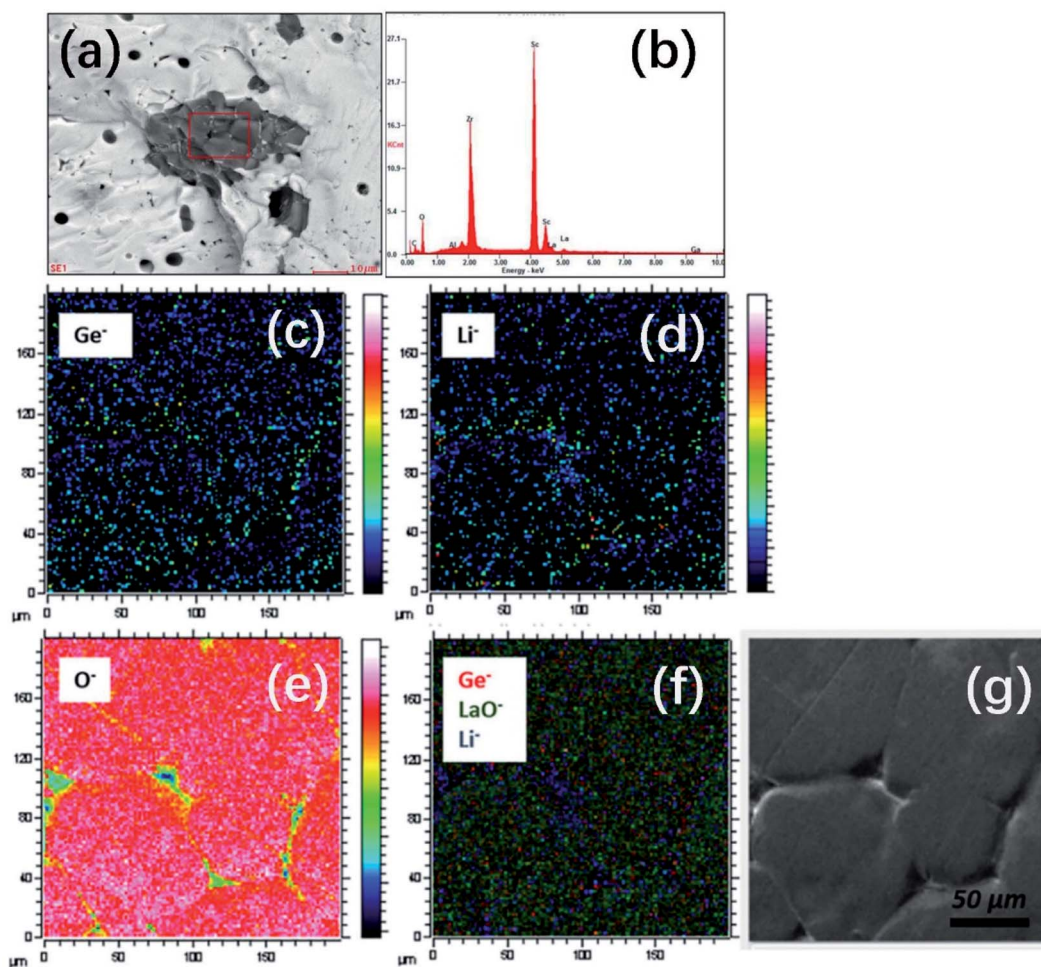
Fig. 5 (a and b) SEM-EDS analysis of the secondary phase observed in LGLZ-Sc. Reproduced with permission from ref. 54. Copyright, 2017, the American Chemical Society. (c–g) TOF-SIMS maps of the \text{Ge}_{0.10} -LLZO ( x = 0.10 ) pellet surface (optical image shown on the far right), showing ^{74}\text{Ge}^- , ^7\text{Li}^- and ^{16}\text{O}^- secondary ion maps of counts of selected species over total ion counts and an overlay of ^{74}\text{Ge}^- , ^{155}(\text{LaO})^- and ^7\text{Li}^- species (in red, green and blue, respectively). Maps were captured with a \text{Bi}^+ primary ion beam (25 kV, 0.2 pA) and a \text{Cs}^+ sputter gun (1 kV, 64 nA) operated in the non-interlaced burst alignment mode (using a 1s:1s:1s sputter:wait:analyse cycle) (for interpretation of the references to color in the figure legend, readers are referred to the web version of this article). Reproduced with permission from ref. 53. Copyright, Clearance Center.
