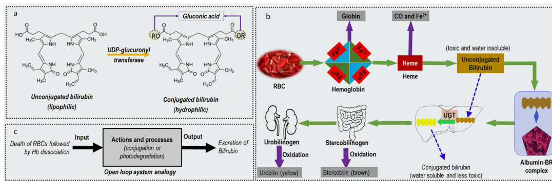
Fig. 1 (a) Bilirubin chemical structure. The left shows the unjugated or indirect bilirubin, whereas the right shows the conjugated or direct bilirubin. The two forms of bilirubin differ from each other with the attached radical after conjugation. (b) Bilirubin pathway: Hb (released from senescent or damaged RBC) breaks down into globin and heme. Heme is then degraded into unconjugated bilirubin (water-insoluble); the latter binds with albumin and is taken to the liver. In the liver, the enzymes act upon UCB to become conjugated bilirubin (water-soluble) which is excreted from the body via stool and urine. (c) An open-loop system analogy of bilirubin excretion. The actions include all the steps involved from the albumin binding to the bilirubin conjugation or the photochemical degradation of bilirubin during phototherapy.
