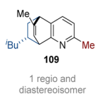
Scheme 31 Dearomative photoredox catalysed intermolecular [4 + 2] cycloaddition of (iso)quinolines. 37
