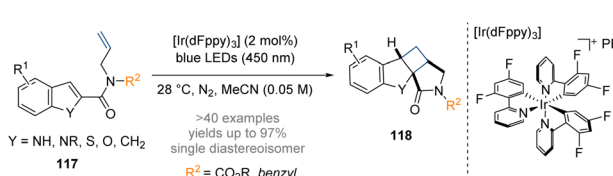
Scheme 34 Dearomative photoredox catalysed intramolecular [2 + 2] cycloaddition of indoles. 40
