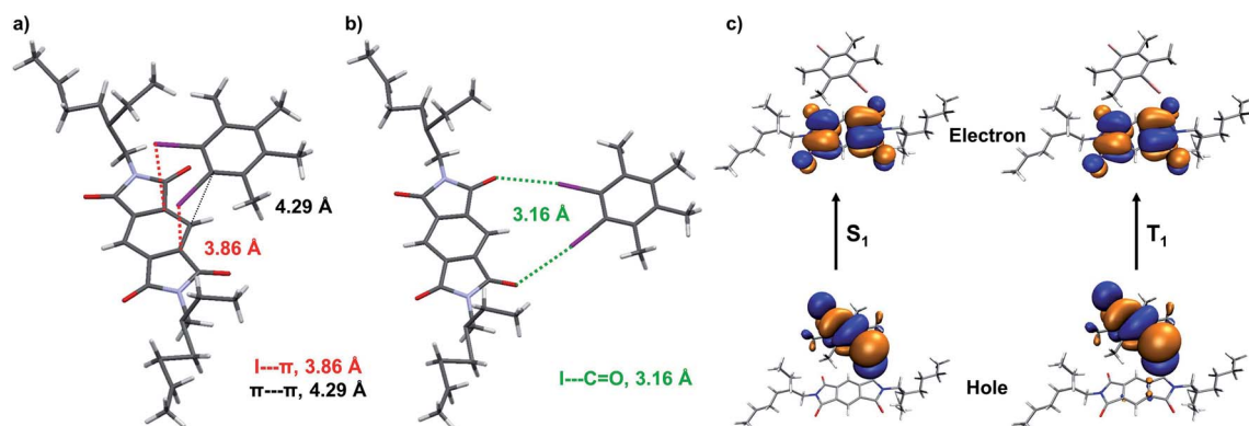
Fig. 4 (a) Single-crystal X-ray diffraction data of A+D 2 co-crystal: donor–acceptor arrangement of A+D 2 pair, driven by various halogen bonding and weak \pi \cdots \pi interactions, such as (a) \text{I} \cdots \pi (marked with red lines), \pi \cdots \pi (marked with black lines) in a stack and (b) \text{I} \cdots \text{C}=\text{O} (marked with green lines) in the same plane. (c) Theoretical calculations of A+D 1 : natural transition orbitals (NTOs) of A+D 1 pair for first excited singlet ( \text{S}_1 ) and triplet state ( \text{T}_1 ), calculated using TD-CAM-B3LYP level in conjunction with 6-31+g(d) basis set for C, N, O, H and LANL2DZ basis set showing CT character.
