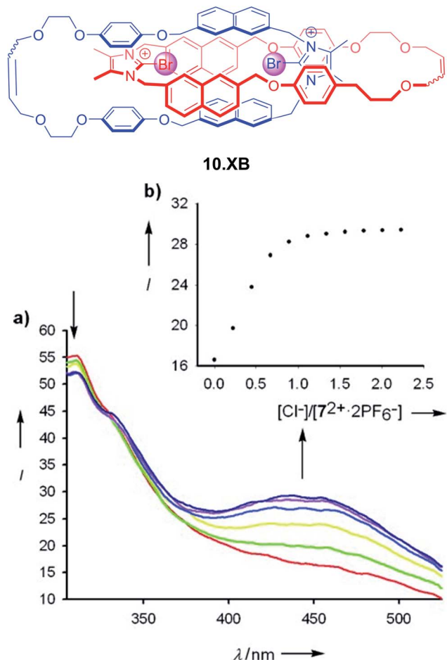
Fig. 13 All-XB bromo-imidazolium-naphthalene catenane 10.XB for fluorescent halide sensing. (a) Emission spectra of 10 \mu\text{M} 10.XB upon addition of Cl - in ACN. (b) The corresponding response isotherm at 445 nm. Reproduced with permission from ref. 122 copyright 2011 Wiley.
