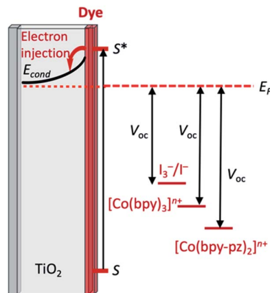
Fig. 3 Schematic illustration of the relative E redox levels (in red) for two representative Co 3+ /Co 2+ redox mediators with respect to the I 3 - /I - couple and the effect on the value of V OC (see Fig. 2a for complete DSC diagram).
