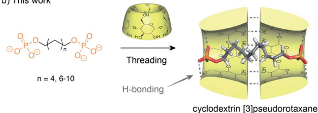
Fig. 1 (a) Previous work on compression of alkyl chains by self-assembled capsules or boxes. (b) Alkyldiphosphate axles used in this study and corresponding CD [3]pseudorotaxane with potential compression resulting from hydrogen bonding and hydrophobic interactions between the threaded axle and head to head CDs.
