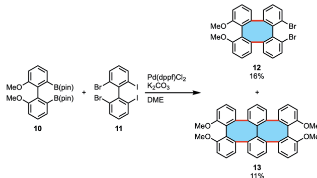
Scheme 4 Double Suzuki–Miyaura coupling of biphenyl diborate 10 and dibromodiiodobiphenyl 11 .
