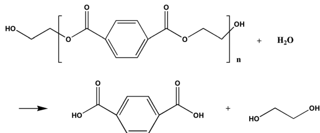
Fig. 4 Reaction formula for the degradation of PET by hydrolysis.
