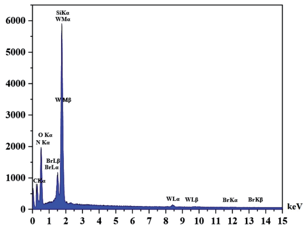
Fig. 4 EDX spectrum of the supported catalyst (Si-1).
