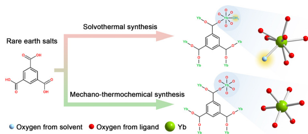
Fig. 1 Illustration of the effect of different synthesis methods on the presence or absence of coordinated solvent molecules in RE-MOFs.
