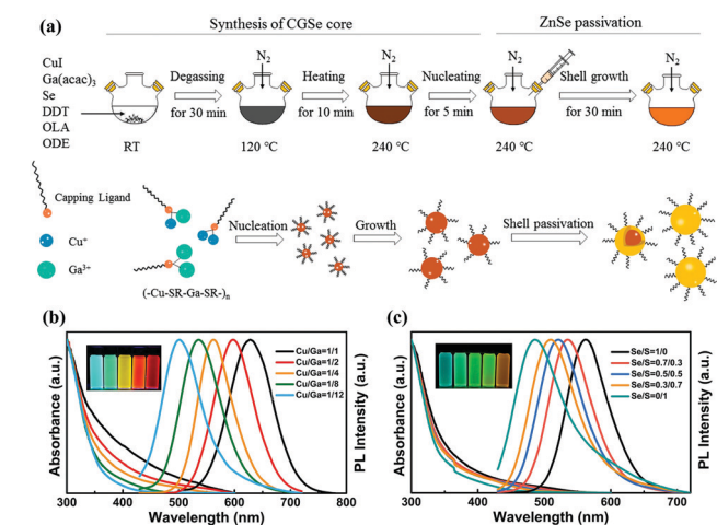
Fig. 4 (a) Schematic illustration of the synthetic procedures of CuGaSe/ZnSe core/shell QDs via a heating-up method. UV-vis absorption (left), PL spectra (right, λ ex = 405 nm) and digital photograph of samples under the radiation of 365 nm UV illumination (inset) of (b) CuGaSe/ZnSe and (c) CuGaSe 1-x /ZnSe QDs prepared under various Cu/Ga and Se/S precursor molar ratios, respectively. Reproduced with permission. 40 Copyright 2018 Elsevier B.V. All rights reserved.
