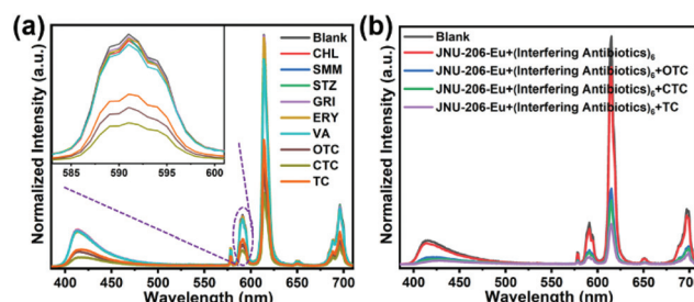
Fig. 4 (a) Luminescence emission spectra of aqueous suspensions of JNU-206-Eu (30 mg per 100 mL) in the presence of different antibiotics (0.5 mM) ( \lambda_{\text{ex}} = 365 nm). (b) Luminescence emission spectra of aqueous suspensions of JNU-206-Eu (30 mg per 100 mL) in the presence of six interfering antibiotics (each 0.5 mM) and further addition of OTC, CTC or TC (0.5 mM), respectively ( \lambda_{\text{ex}} = 365 nm).
