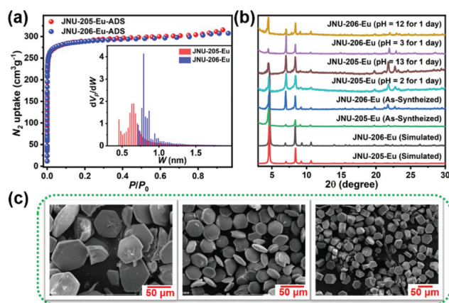
Fig. 2 (a) \text{N}_2 adsorption isotherms of JNU-205-Eu and JNU-206-Eu at 77 K. Inset shows pore size distribution plots according to the HK method. (b) Comparison of the simulated PXRD patterns with the experimental ones of the as-synthesized JNU-205-Eu / JNU-206-Eu and after being treated with base (pH = 12, 13) or acid (pH = 2, 3) for one day. (c) Representative desktop scanning electron microscope (SEM) images of JNU-206-Eu (left), JNU-206-Y (middle) and JNU-206-Nd (right).
