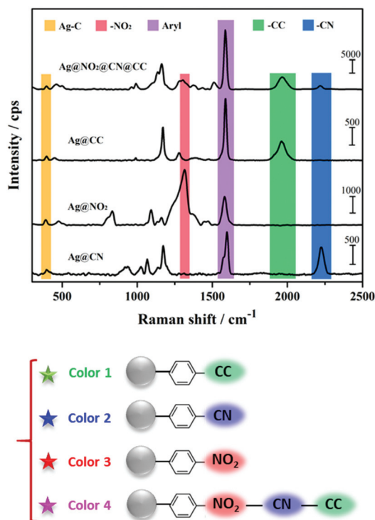
Fig. 5 SERS spectra of the three single layer-SERS tags and multilayer-coated Ag@NO 2 @CN@CCH NPs. The excitation wavelength was 638 \text{ nm} , and the exposure time was 2 \text{ s} . The molecular structures of the three Raman reporters derived from aryl diazonium salts and the multilayer-coated Ag@NO 2 @CN@CCH NPs are illustrated below.
