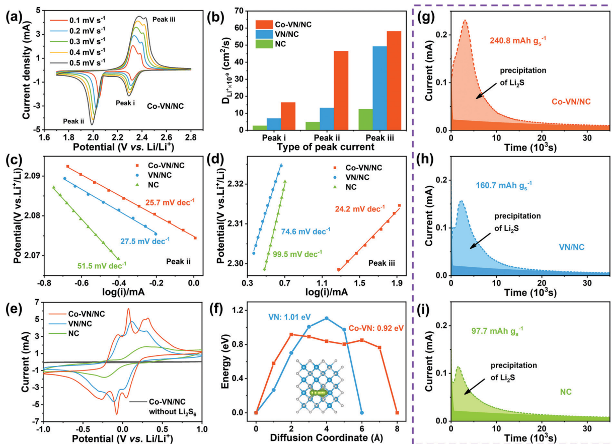
Fig. 5 (a) CV curves of Co-VN/NC electrodes at scan rates from 0.1 to 0.5 \text{mV s}^{-1} . (b) Diffusion coefficient of \text{Li}^+ ions of Co-VN/NC, VN/NC and NC electrodes for peak i, ii, and iii processes. (c and d) Tafel plots corresponding to peak ii and iii with the different cathode composites. (e) CV curves obtained at 1 \text{mV s}^{-1} for the \text{Li}_2\text{S}_6 symmetric cells using Co-VN/NC, VN/NC and NC as electrodes, respectively. (f) Energy barriers of \text{Li}^+ diffusion on the Co-VN and VN (200) plane. (g–i) Potentiostatic discharge curves of \text{Li}_2\text{S}_8 solution on the surfaces of the Co-VN/NC, VN/NC and NC.
