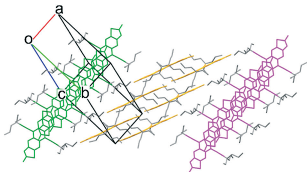
Fig. 4 Crystal packing of EDnPC-FADT, where molecules of the same color are electronically communicative with one another.
