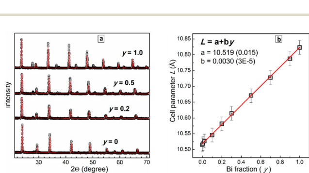
Fig. 2 (a) X-Ray diffractograms of CANBIC perovskites with x = 0.4 and y = 0, 0.2, 0.5, and 1.0 . Gray circles correspond to experimental data, red solid lines are the results of Rietveld refinement. (b) Cell parameter of CANBIC perovskites as a function of Bi fraction y . Gray squares are experimental data, red line represents a linear fit (fitting parameters a and b are presented in figure).
