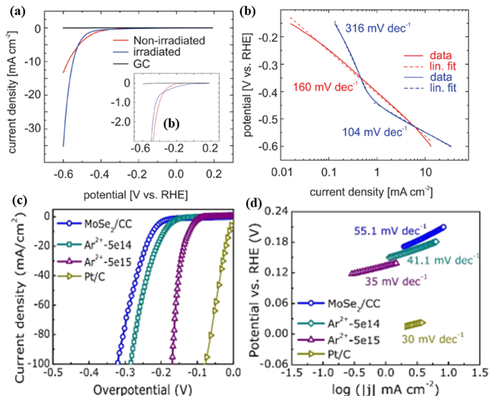
Fig. 9 (a) Current density as a function of the potential (V vs. RHE) showing strong activity enhancement of the irradiated MoSe 2 compared to that of the non-irradiated MoSe 2 . The inset of (a) shows the less negative onset potential for the irradiated MoSe 2 . (b) V – I curves with Tafel-slopes of the irradiated (blue) and non-irradiated (red) MoSe 2 . Reproduced with permission from ref. 65. Copyright 2018, Royal Society of Chemistry. The HER performance of the as-fabricated catalysts. (c) LSV curves and (d) Tafel plots of MoSe 2 /CC, Ar 2+ -5e14, Ar 2+ -5e15 and Pt/C electrodes, respectively. Reproduced with permission from ref. 66. Copyright 2018, American Chemical Society.
