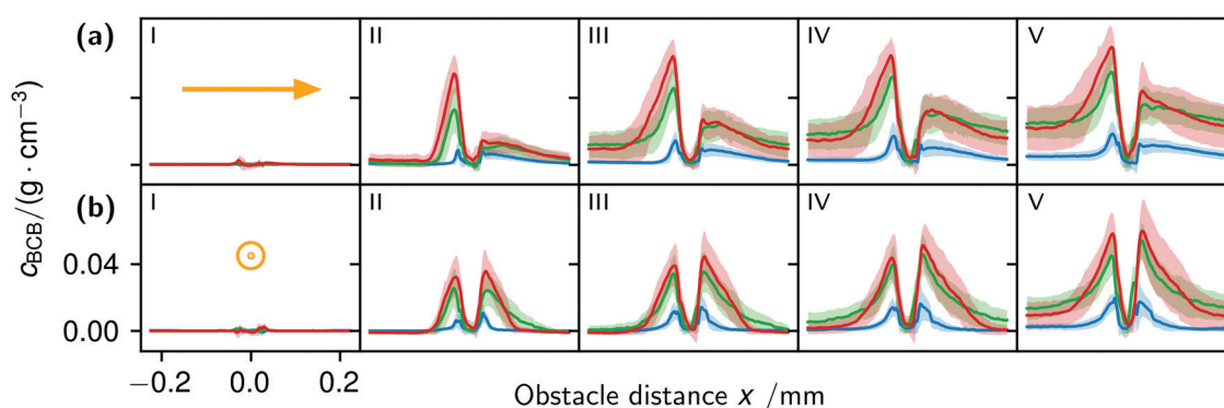
Fig. 8 Profile plots parallel (a) and perpendicular (b) to the flow in timesteps I–V of 7.5 h, whereby timestep I was 10 minutes after the start. The obstacle center is the x -axis center and fluid flow is indicated by the orange arrows. The blue line represents flow at 1.0 \text{ mm s}^{-1} , the green line at 12.5 \text{ mm s}^{-1} and the red line at 25.0 \text{ mm s}^{-1} .
