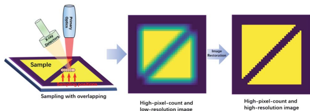
Fig. 1 Diagram of acquiring a high-resolution image with over-sampling mapping and image restoration techniques.
