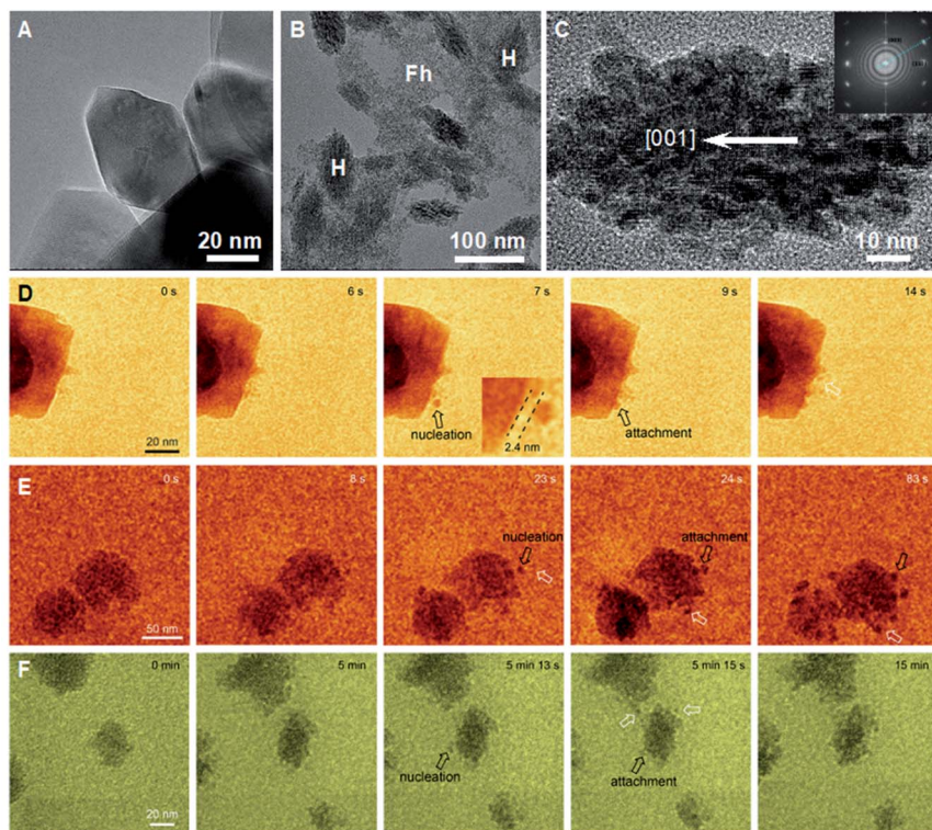
Fig. 7 (A–C) Ex situ TEM data showing (A) rhombohedral Hm formed during dissolution-precipitation from Fh in oxalate free solution; (B) Hm (H) spindles forming in a Fh (F) suspension containing sodium oxalate; (D–F) in situ TEM data showing the near-surface nucleation and attachment of Hm nanoparticles (D and E) during the initial period of Hm particle formation and (F) over an extended time period to show the development of Hm spindles. 80 Reproduced from ref. 80 with permission from Springer Nature. Copyright 2021.
