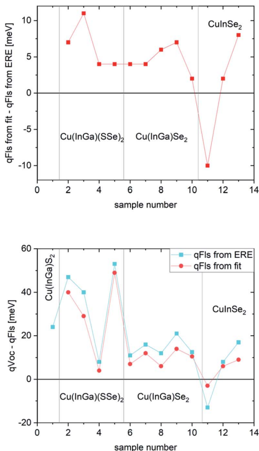
Fig. 4 Comparison for various chalcopyrite solar cells. (Top) difference between qFls determined by the two different methods. (Bottom) Comparison between V_{\text{OC}} and qFls.
