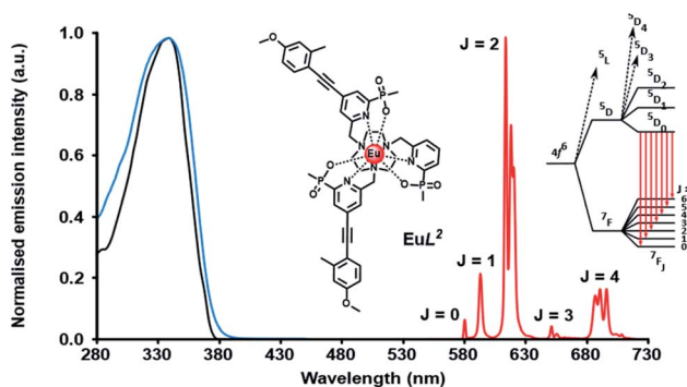
Fig. 2 Absorption (blue), excitation (black) and emission ( \lambda_{\text{exc}} 355 nm; red) spectra of [EuL 2 ], showing the five major transitions to the ^7F_n ground state from the europium ^5D_0 excited state, (295 K, 0.1 M NaCl).
