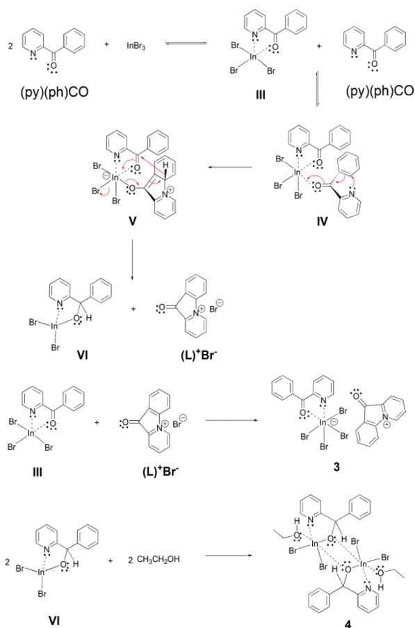
Scheme 4 The proposed mechanism for the formation of complexes (\text{L})[\text{InBr}_4\{(\text{py})(\text{ph})\text{CO}\}] ( 3 ) and [\text{In}_2\text{Br}_4\{(\text{py})(\text{ph})\text{CH}(\text{O})\}_2(\text{EtOH})_2] ( 4 ).
